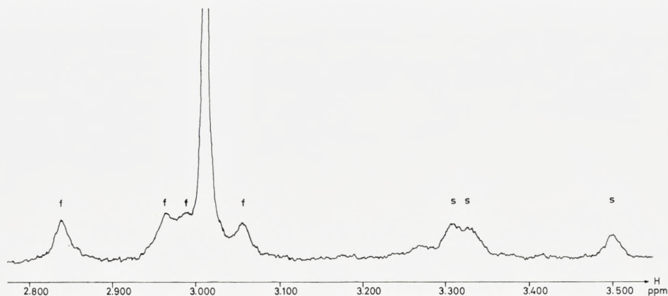
Fig. 1. 10 accumulated FMR spectra of hepta-trifluoroacetylated glucagon in \text{CF}_3\text{COOH} . f = 'fast' -\text{CH}_2\text{OCOCF}_3 resonance, s = 'slow' >\text{CHOCOCF}_3 resonance. The strong line at 3.01 ppm/internal \text{CFCl}_2\text{CF}_2\text{Cl} is the ^{13}\text{CF}_3\text{COOH} low-field spin satellite.
